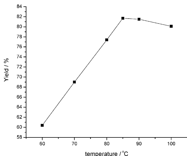
Figure 2. The effect of temperature on the nitration of toluene. Toluene and \text{HNO}_3 (95%) = 3 mmol; reaction time 4 h; 2 mol% \text{La}(\text{NTf}_2)_3 as catalyst; yields were determined by quantitative GC analysis.
